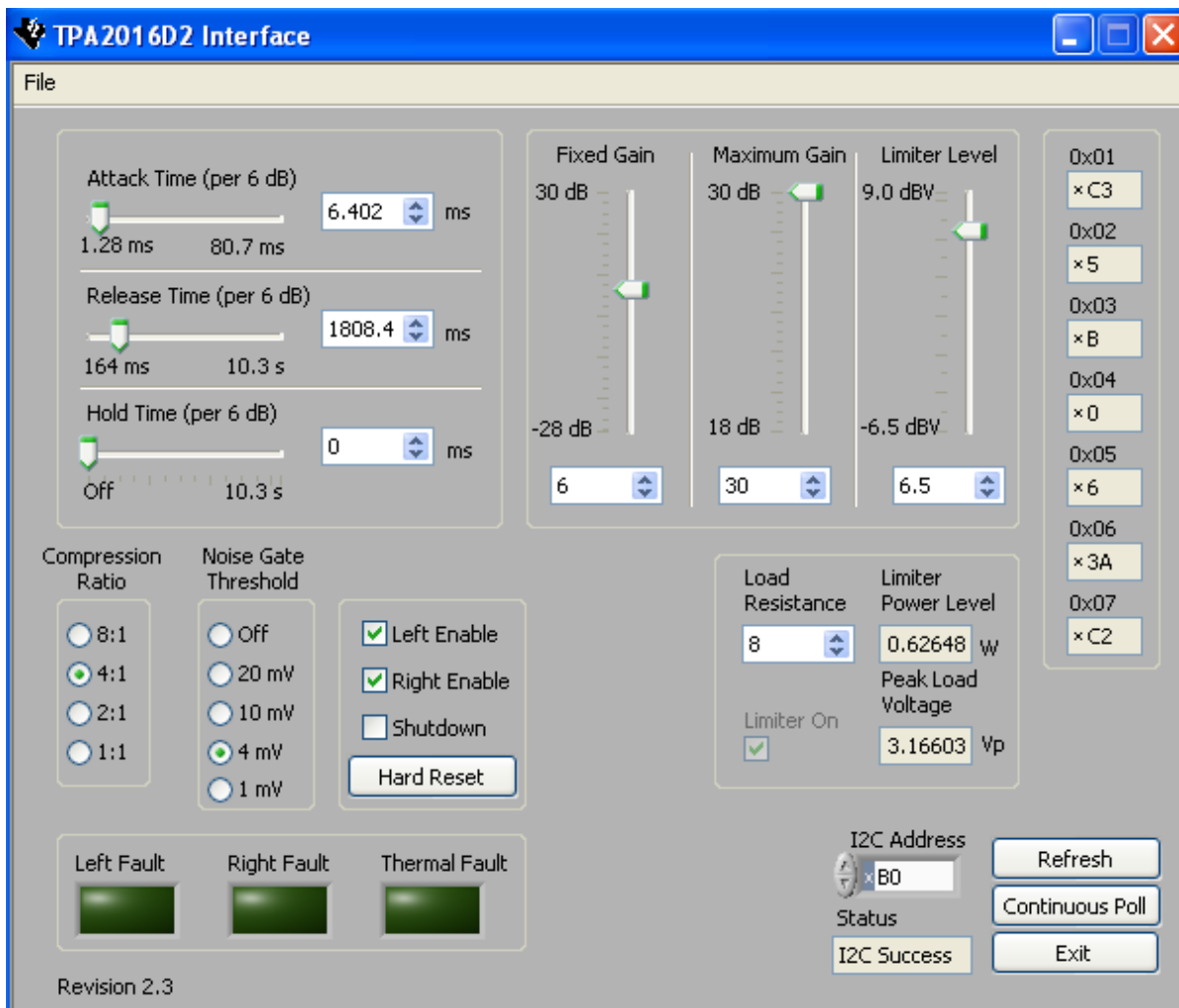
Figure 4. Software Interface
