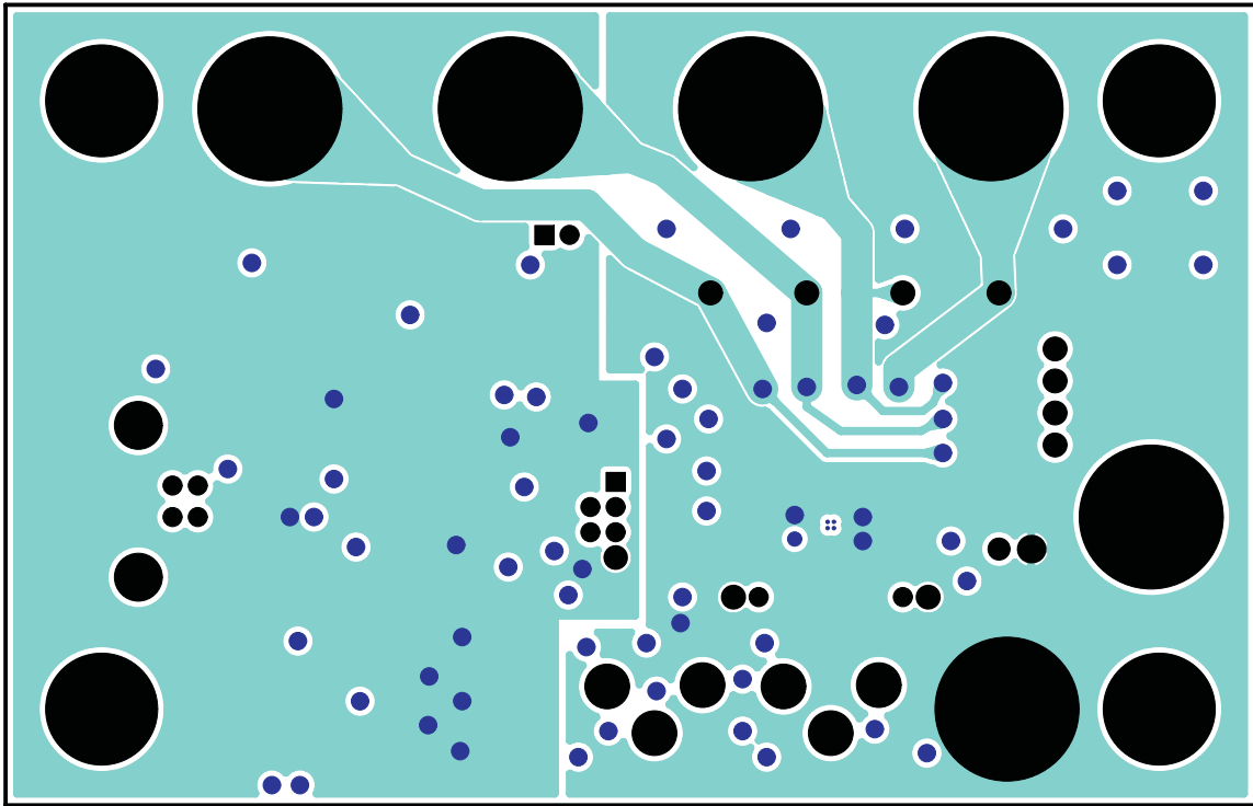
Figure 9. TPA2016D2EVM – Layer 3
